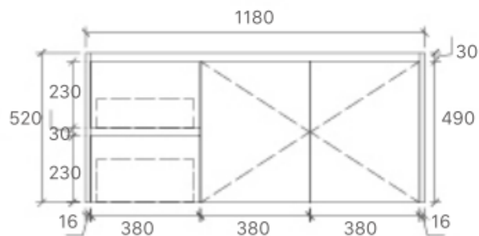
SYWH05-1200L Size: 1180x455x520mm
