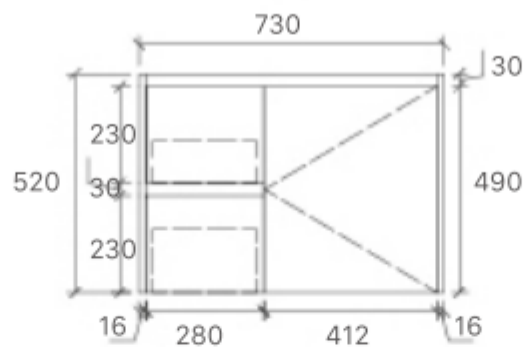
SYWH05-750L Size: 730x455x520mm
