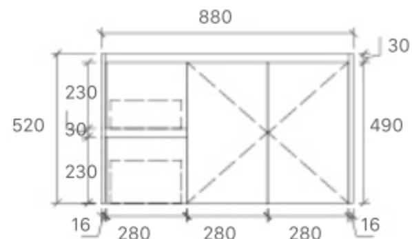
SYWH05-900L Size: 880x455x520mm
