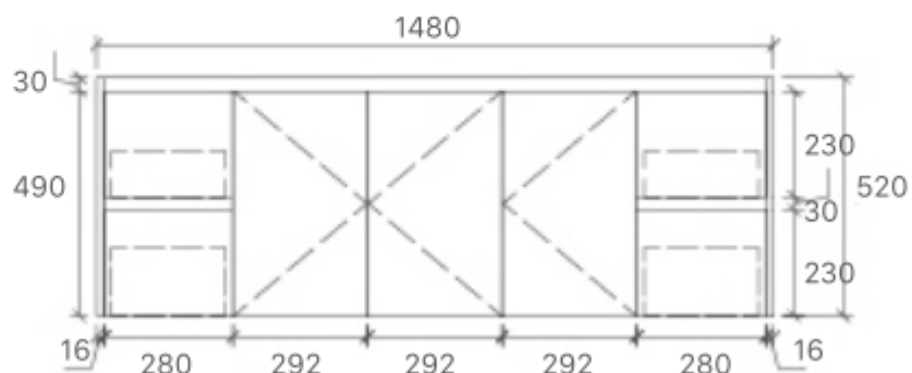
SYWH05-1500 Size: 1480x455x520mm
