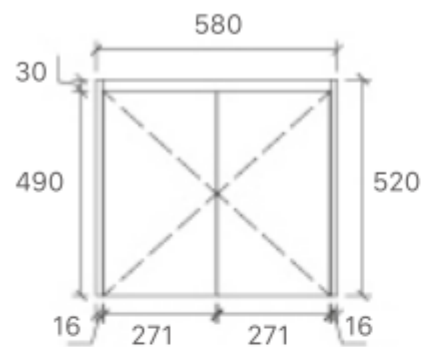
SYWH05-600 Size: 580x455x520mm
